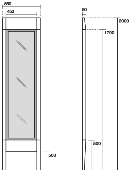
9182 Specchio a terra 55x200x5 cornice legno Floor standing mirror 55x200x5 w/wooden frame
